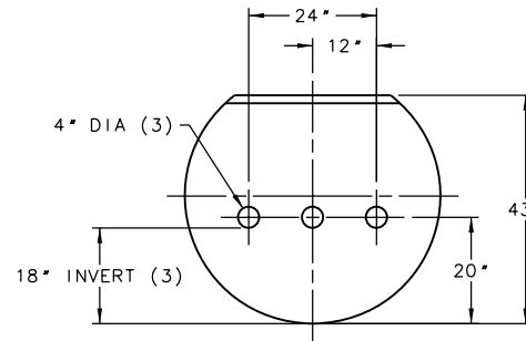
BAFFLE DETAIL
